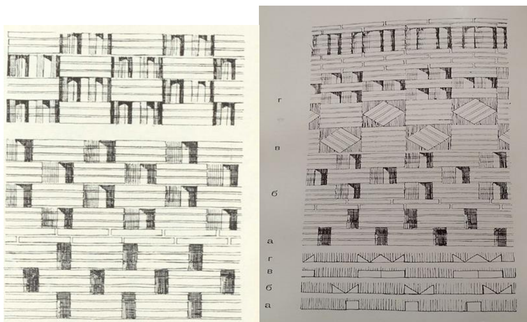
Fig 2: Brick construction methods on the walls inside and outside of the Samanid Mausoleum
